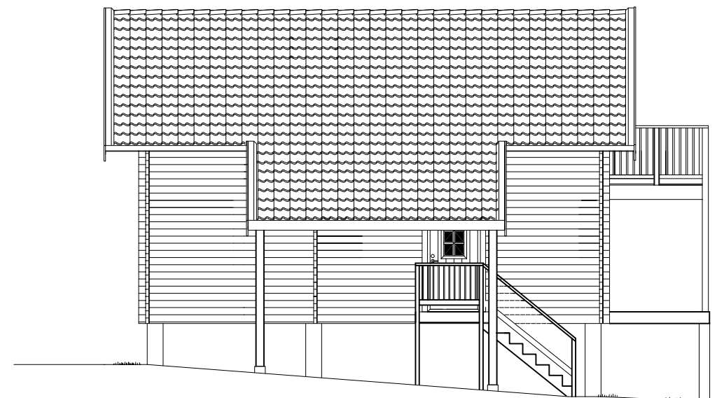
SIDE FACADE
