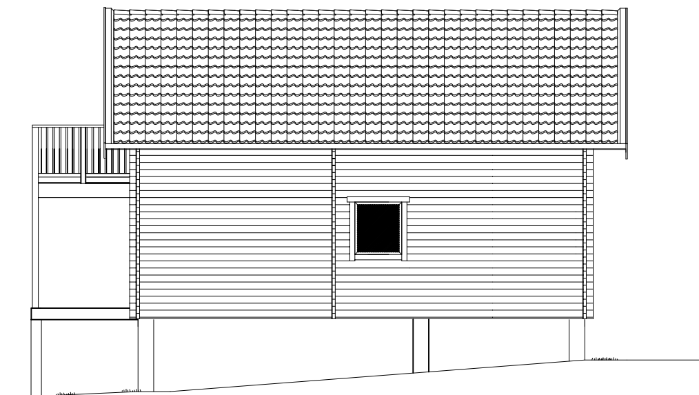
SIDE FACADE
